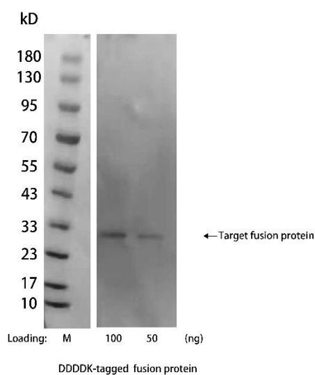
Figure 1. Detection of DDDDK tag in recombinant fusion protein were analyzed by Western blot using Rabbit Anti DDDDK Tag Antibody, pAb(Cat.DTA0198, at 1 \mu\text{g/mL} concentration).
